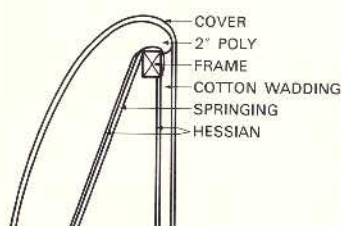
TYPICAL BACK REST SECTION (FROM SIDE)
