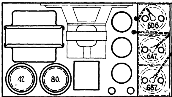
Fig. 1.—Showing position of Valves and location of Grid Leads.
