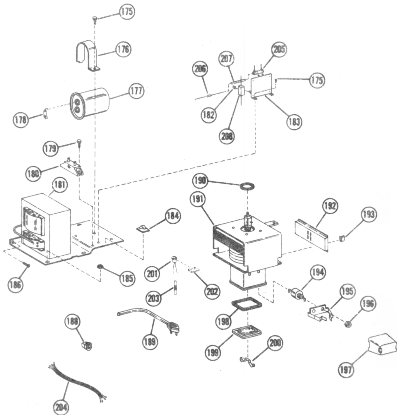
ELECTRICAL PART.
