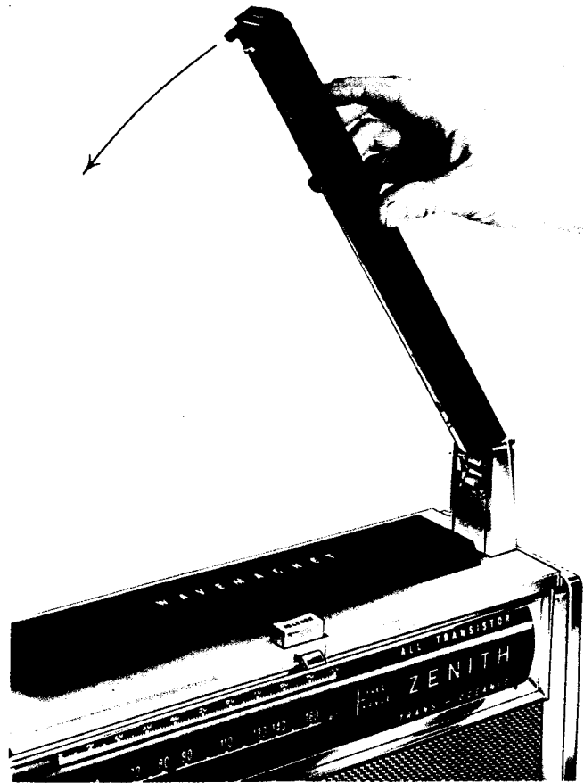
FIGURE 9 LOWERING THE HANDLE
