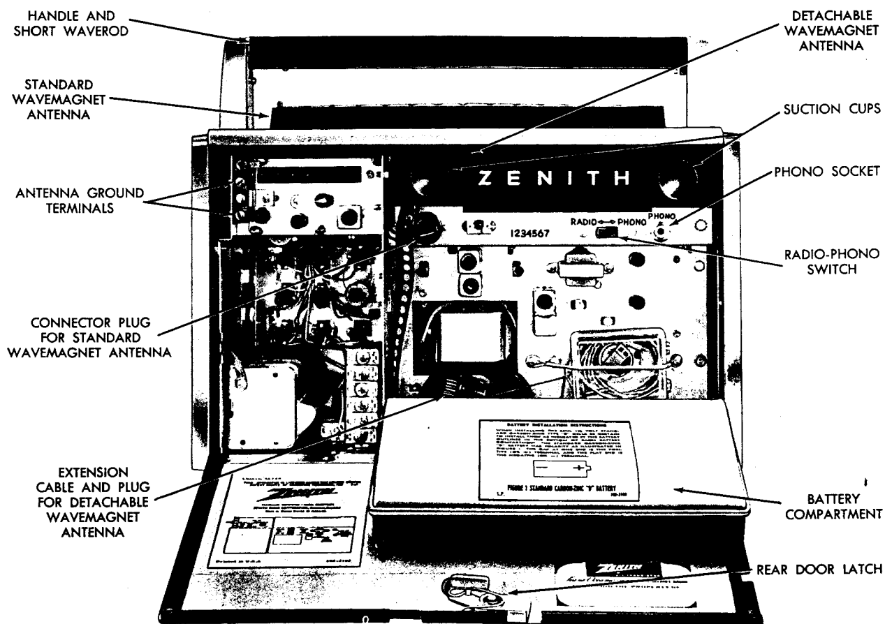
FIGURE 1 REAR VIEW BACK COVER OPEN
